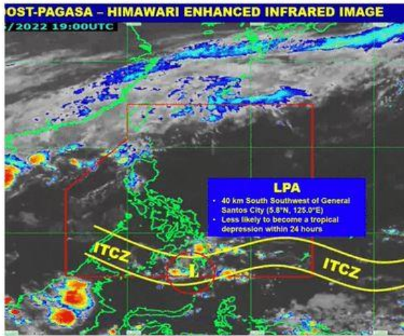
4 AM UPDATE 02 MAY 2022 MONDAY DOST-PAGASA HIMAWARI E-IR IMAGE
