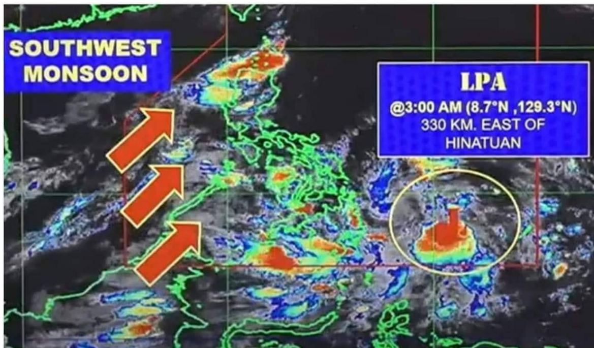
DOST-PAGASA HIMAWARI E-IR IMAGE
