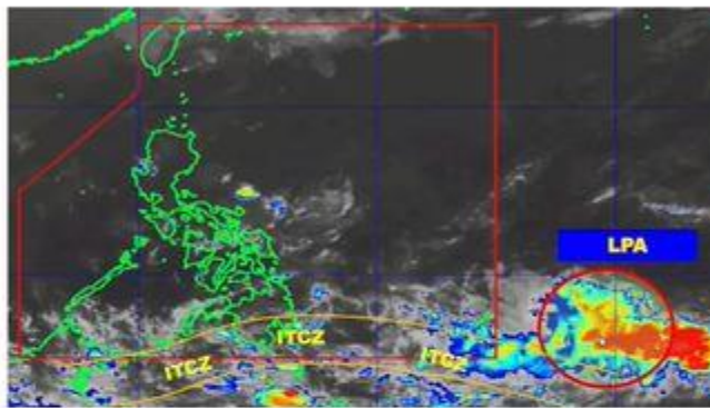
DOST-PAGASA HIMAWARI E-IR IMAGE
